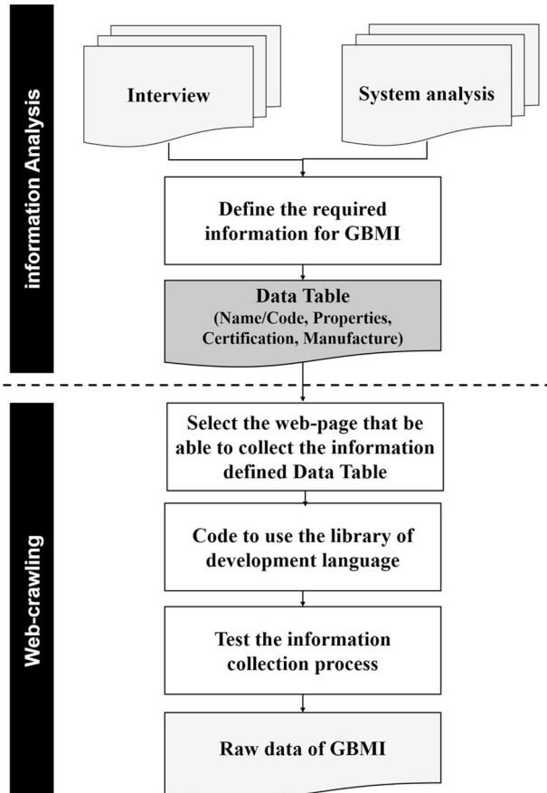
Fig. 4. Information collection process using web crawling.
