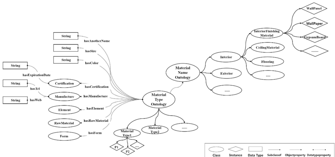
Fig. 5. The structure of green building material ontology.
