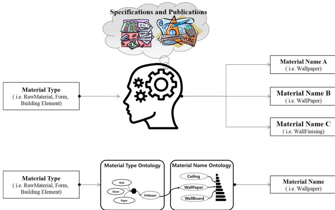
Fig. 2. Concept of ontology inference.
