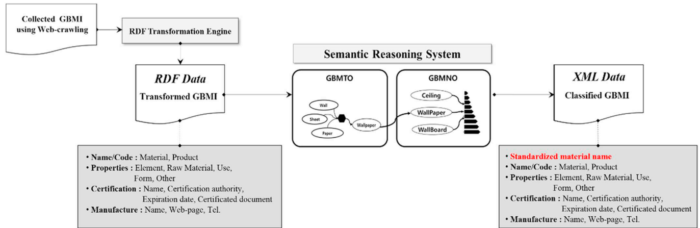
Fig. 6. Information classification process using ontology.
