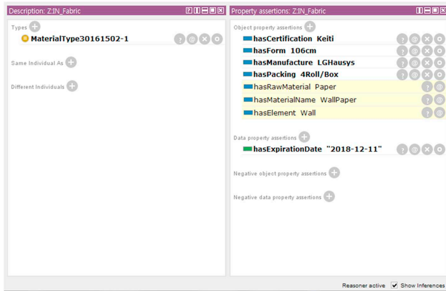
Fig. 9. Results of reasoning information using ontology.
